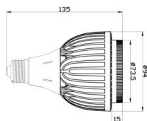
Dimension ( mm )
